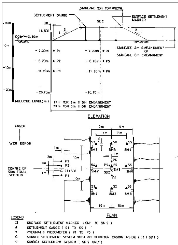
Figure 12 : Layout of Instrumentation Scheme (MHA, 1989)
