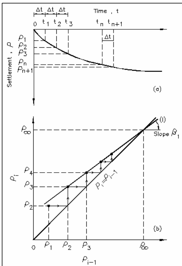
Figure 17 : Graphical Method of Asaoka
