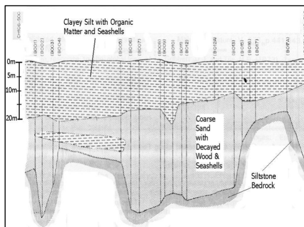
Figure 3 : Geological Cross-Section near Butterworth of the North-South Expressway (Raj & Singh, 1990)
