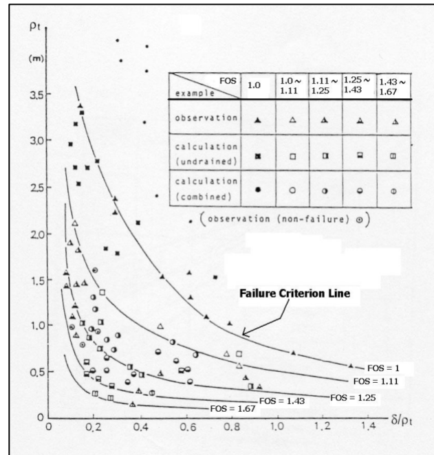
Figure 13 : Modified Matsuo Stability Plot
