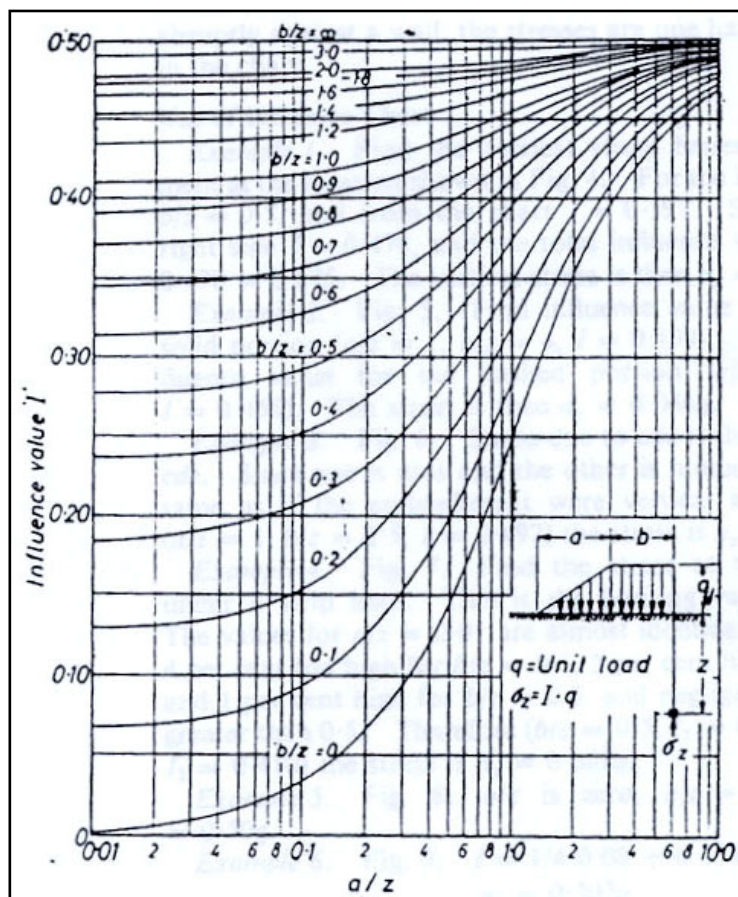
Figure 3 : Influence Chart for Vertical Stress Embankment Loading – Infinite Extent (from Osterberg, 1957)
