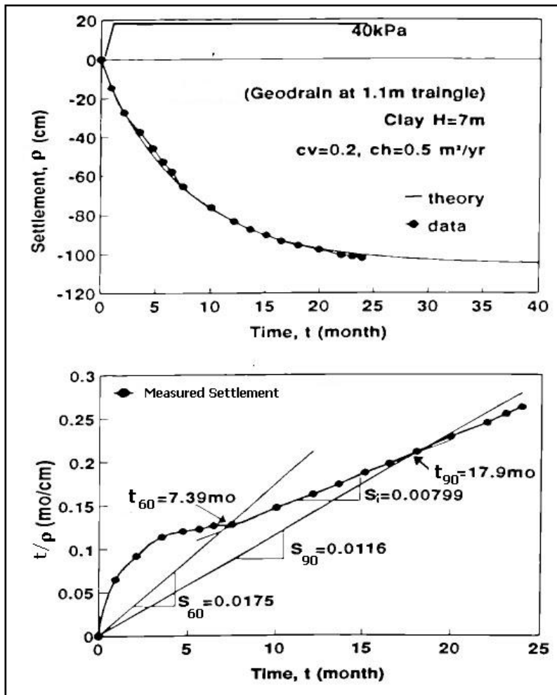
Figure 15 : Example of Hyperbolic Plot Method (Adapted from Tan et. al., 1996)
