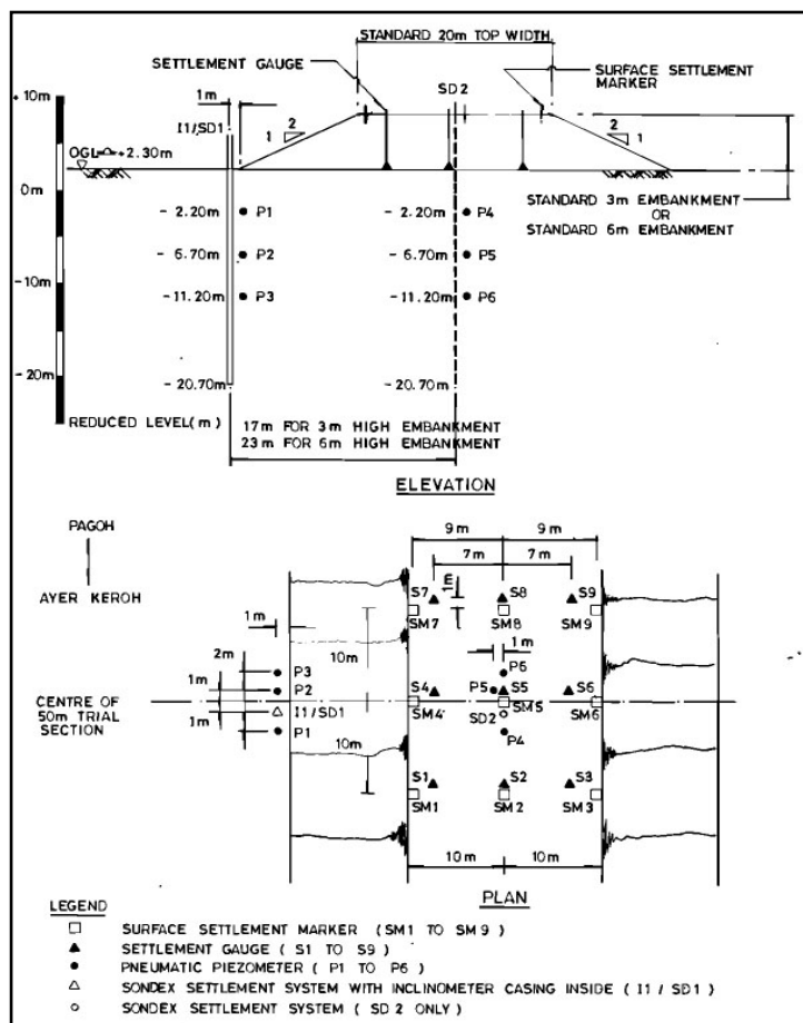
Figure 11 : Layout of Instrumentation Scheme (MHA, 1989)
