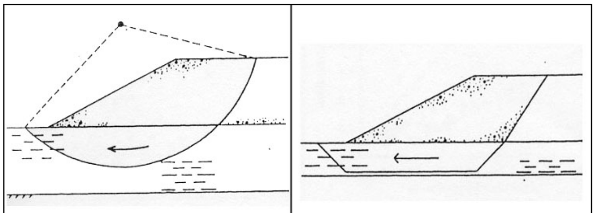
Figure 2 : Circular & Non-Circular Failure Surfaces
