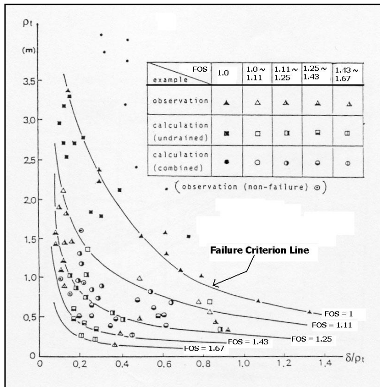
Figure 12 : Modified Matsuo Stability Plot
