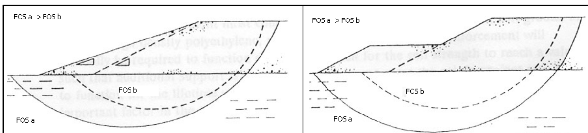
Figure 9 : Improvement of Embankment from Reduction in Slope Angle or using Berms
