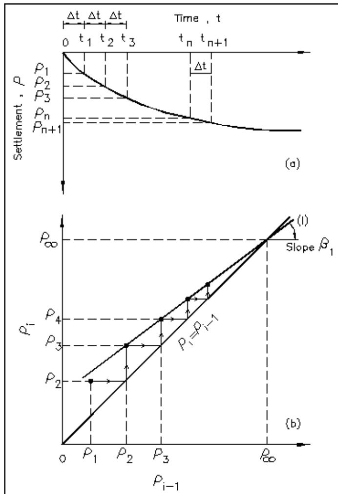
Figure 16 : Graphical Method of Asaoka
