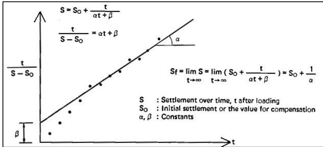
Figure 13 : Hyperbolic Method to Predict Future Settlement
