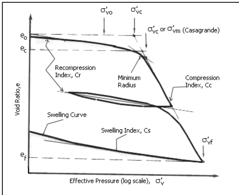
Figure 4 : Notation and Terminology used for Oedometer Compression Curves (from Balasubramaniam & Brenner, 1981)
