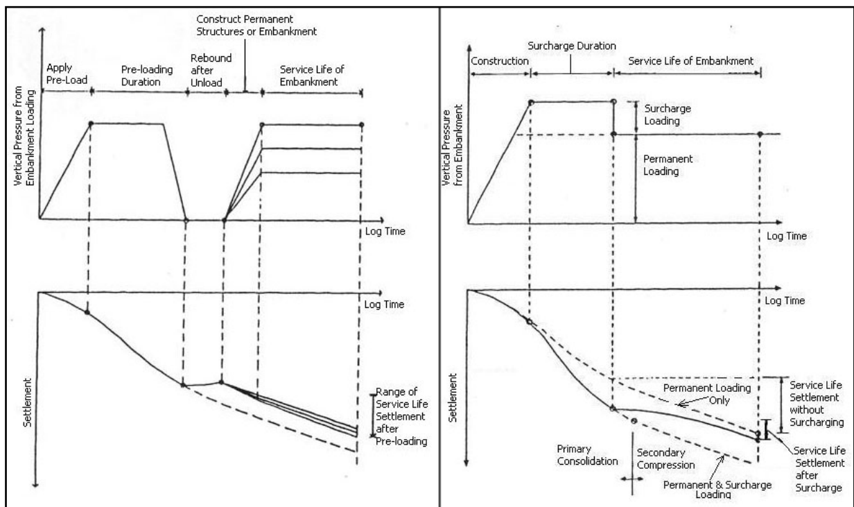
Figure 10 : Concept of Pre-Loading and Surcharge
